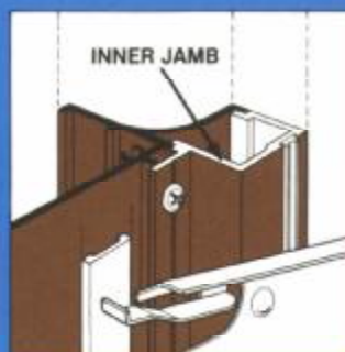
SECTION THROUGH JAMB
